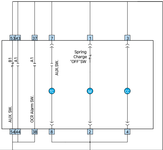
“Stand-by” Circuit Breaker’s Auxiliary Device
