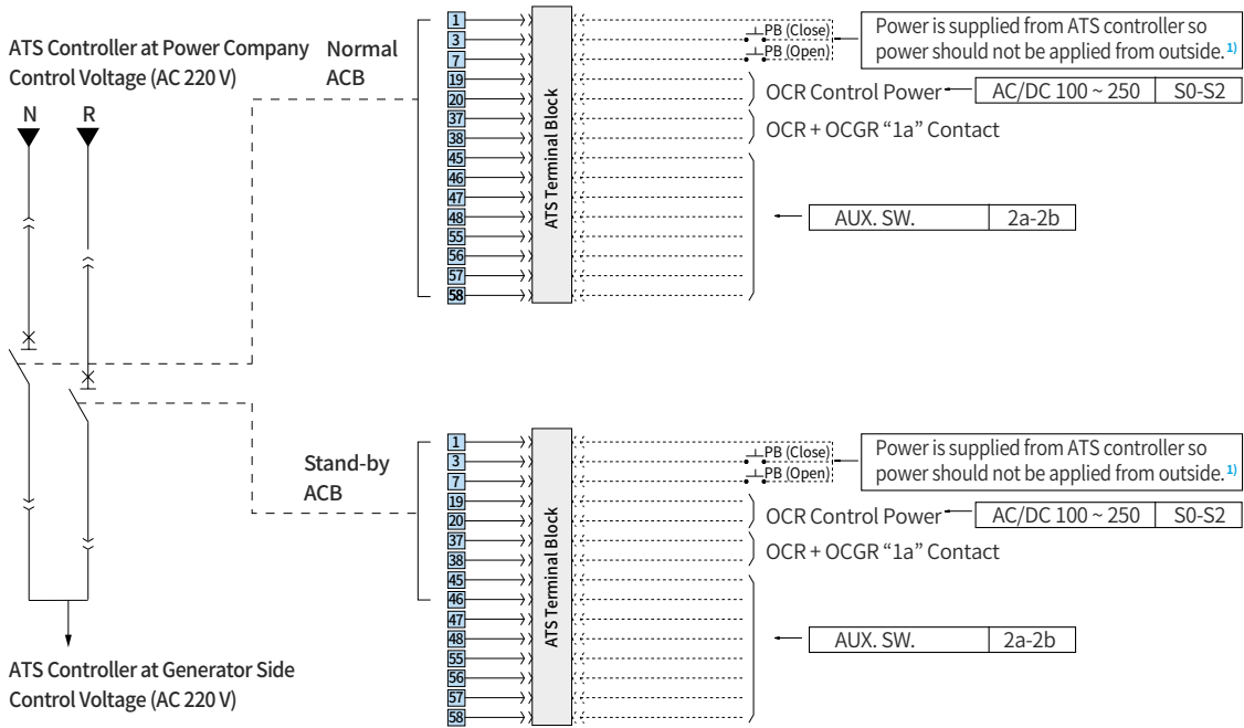
ATS Panel Remote Circuit Diagram
